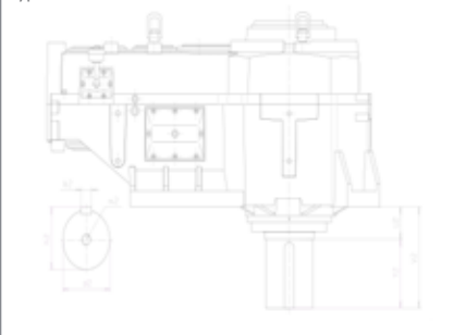
Solid shaft downwards
