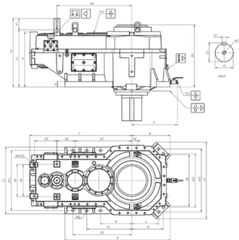
Gear unit dimensions, type D3PVSF
