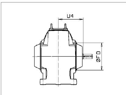
Fan, page 12.21
