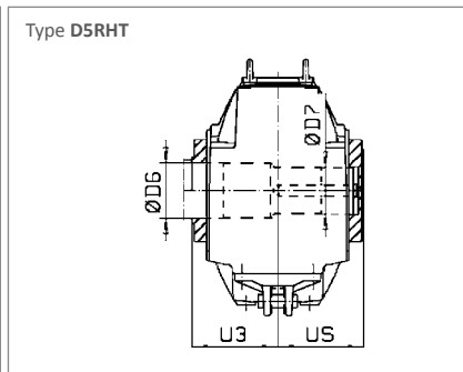
Hollow Shaft, Special Key Connection, page 12.12
