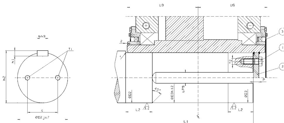
Shaft end
