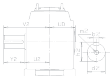
Solid shaft
