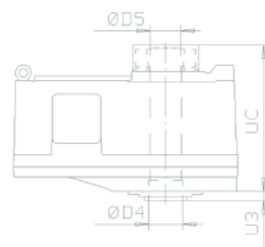
Hollow shaft, shrink disk, page 12.13
