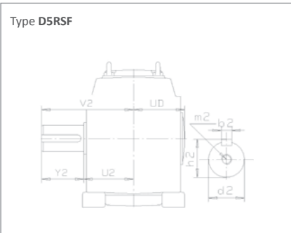
Solid shaft
