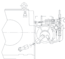
Lubrication unit, page 12.23
