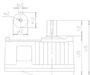
Solid shaft upwards
