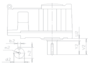
Type D4PVSF
