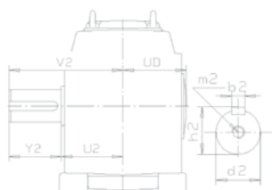
Solid shaft
