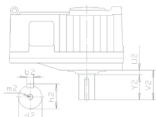
Solid shaft downwards
