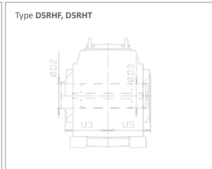
Hollow shaft, key connection, page 12.10
