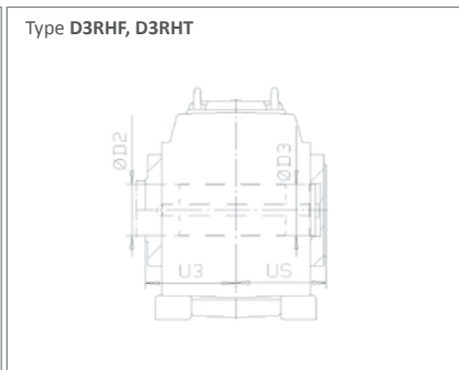
Hollow shaft, key connection, page 12.10
