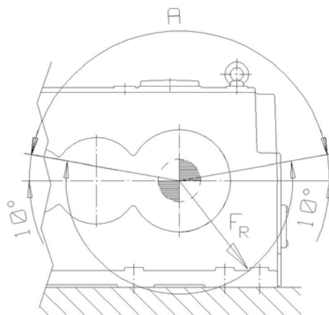
Picture 2: Allowed radial load directions
