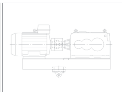
Swing base for motor, page 12.36
