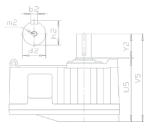
Solid shaft upwards
