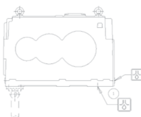
Oil drain plugs position D2P., D3R..
