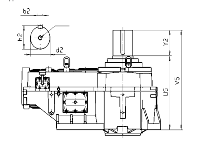
Solid shaft upwards
