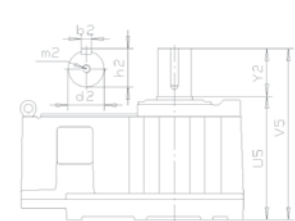
Solid shaft upwards
