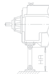
Torque arm, page 12.31
