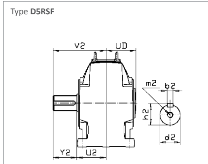
Solid shaft
