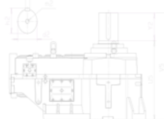
Solid shaft upwards
