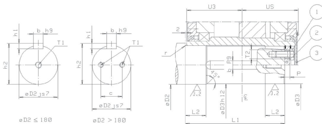
Shaft end
