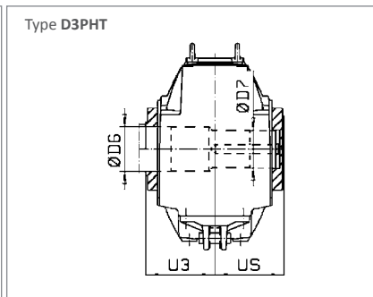
Hollow shaft, special key connection, page 12.12
