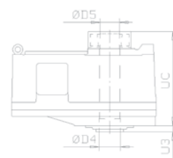
Hollow shaft, shrink disk, page 12.13
