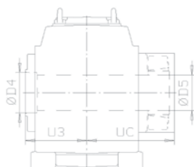
Hollow shaft, shrink disk, page 12.07
